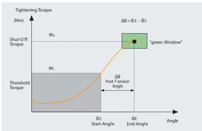
Angle-controlled tightening
