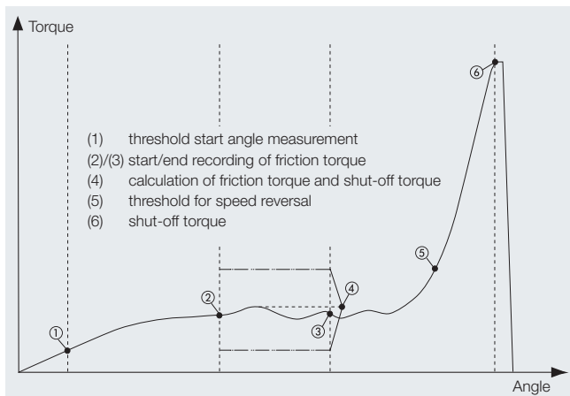
Angle-controlled tightening
